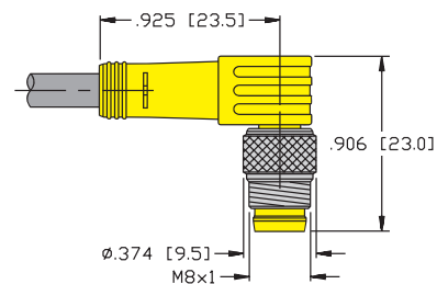
Male Connector, Threaded
