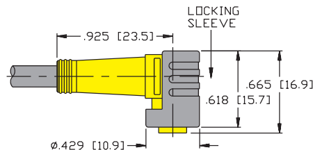
Female Connector, Snap Lock
