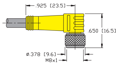
Female Connector, Threaded
