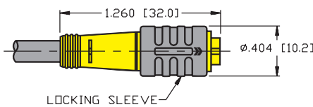
Female Connector, Snap Lock
