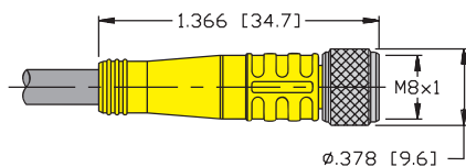
Female Connector, Threaded
