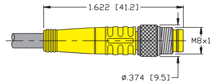
Male Connector, Threaded
