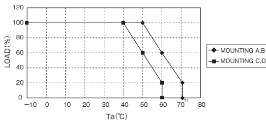
OUTPUT DERATING CURVE
