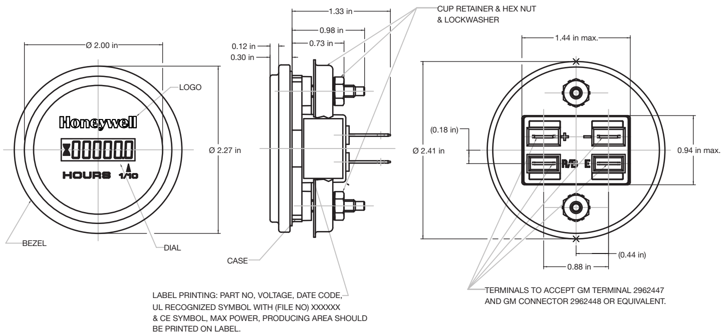
Figure 3. Round-Shaped Hour Meter Dimensions
