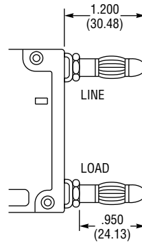
Mounting Pin
