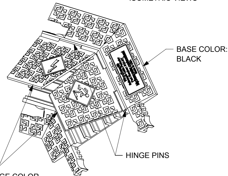
ISOMETRIC VIEWS
