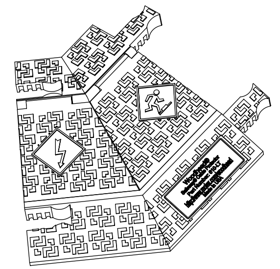
ISOMETRIC VIEWS
