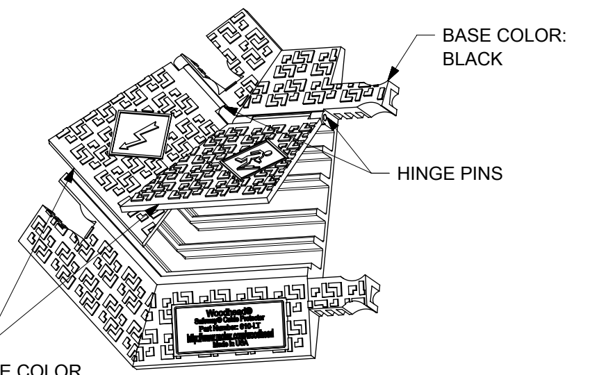
ISOMETRIC VIEWS
