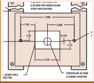
Applicator Ordering Guidelines & Press Specifications
