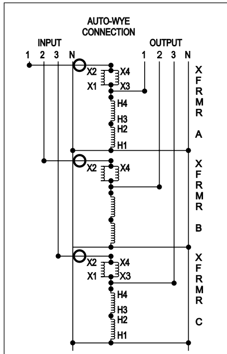
Diagram L2 – Bucking
