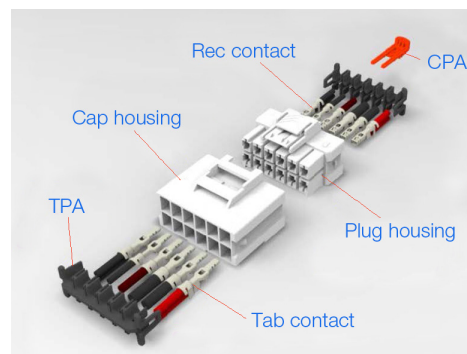
Figure 1. Product design components of the POWER TRIPLE LOCK connector. (2 rows as shown, single row and triple rows excluded here)
