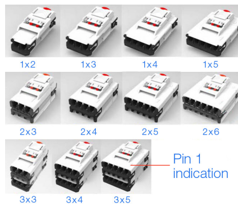
Figure 3. Examples of PTL position configurations.
