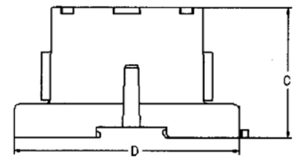
PDBFS500
